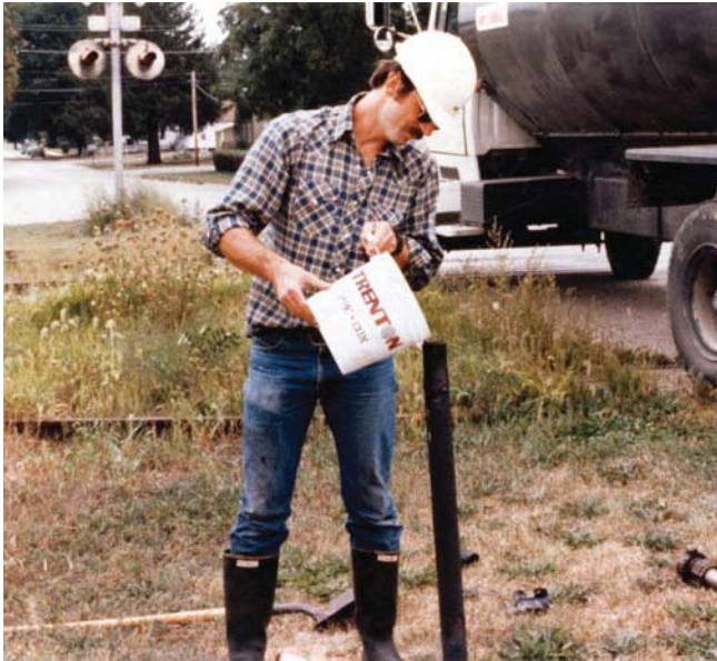
Pre-Con being poured into the casing through the casing vent.
