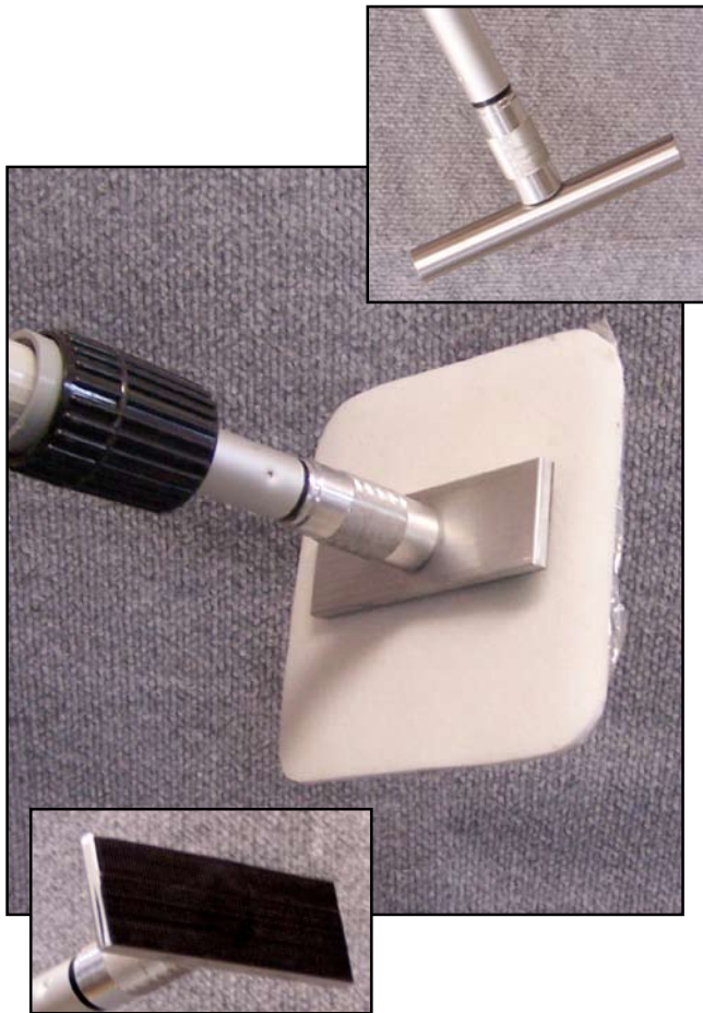
The Trenton Keyhole Patch-Pad applicator tool has a velcro surface (left) for holding the Patch-Pad. The center picture shows the applicator tool with an attached Patch-Pad that has pre-applied coating. The finishing tool (right) is used to press the Patch-Pad onto the pipe.
